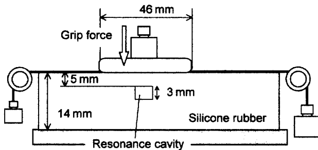
Fig. 10: Experimental setup using ARTC [4,5] tactile device.
