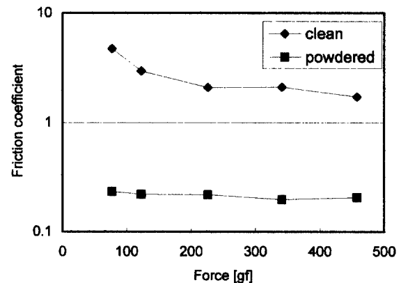
Fig. 11: Friction coefficients of the two samples. A clean acrylic surface and talcum-powdered surface of the same size and material.
