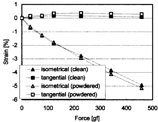
Fig. 12: Measured strains (extensions) of the resonant cavity.
