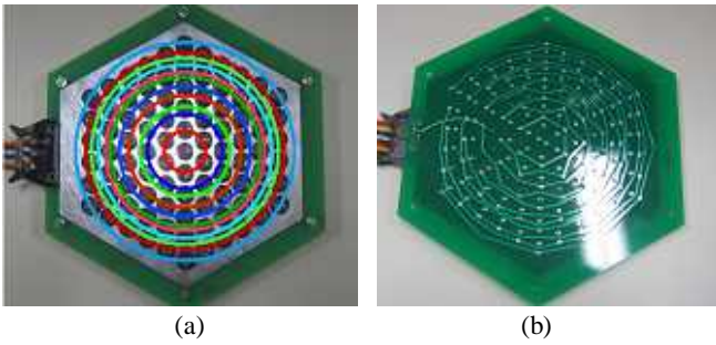
Fig.3 Annular array: (a) front side (b) back side
