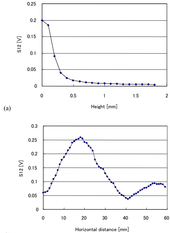
Fig. 10. Measured S12 versus connector position. S12 versus vertical displacement of the connector (a), and S12 versus horizontal displacement of the connector (b).
