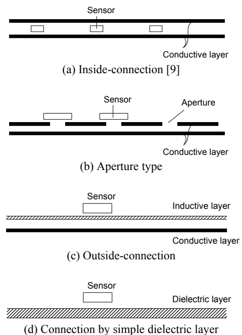
Fig. 2. Cross-sections of possible types of 2DST. In this paper, types (c) is studied.
