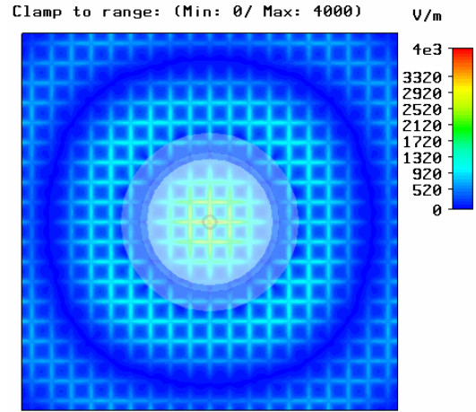
Fig. 7. Simulation results. The cross-section view of electric field intensity around the proximity connector (a), and the top view (b).
